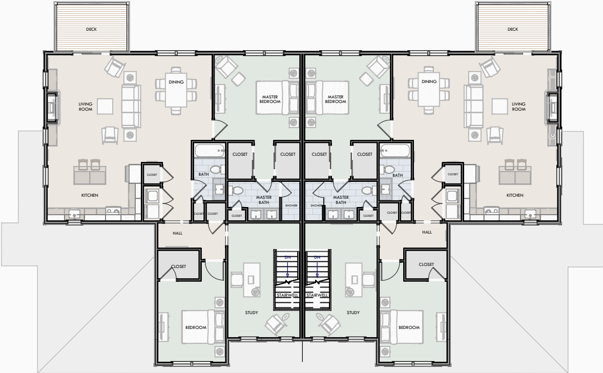
SECOND FLOOR PLAN - 1,680 SF PER UNIT
