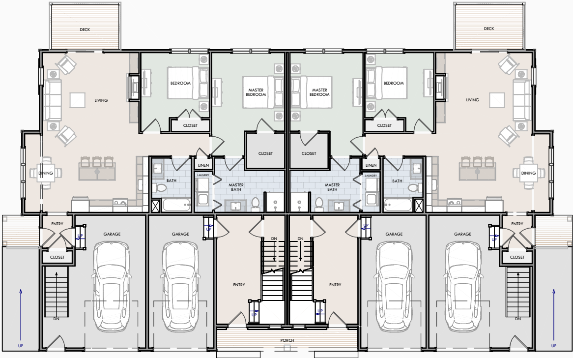
FIRST FLOOR PLAN - 1,265 SF PER UNIT
