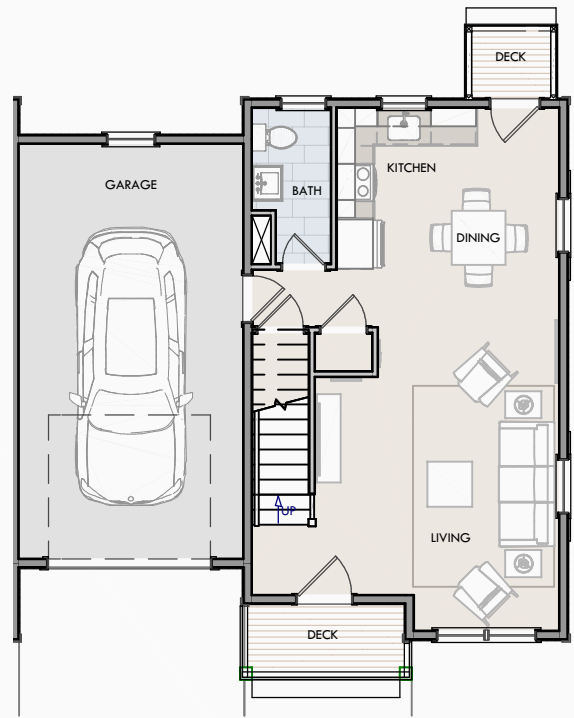
FIRST FLOOR PLAN - 522 SF
